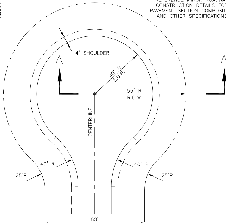
SWALED SECTION
