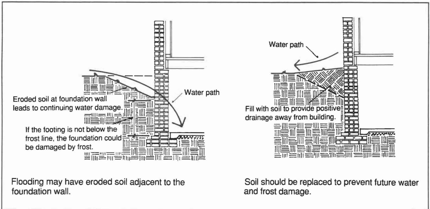
Figure 2. Foundation Erosion
