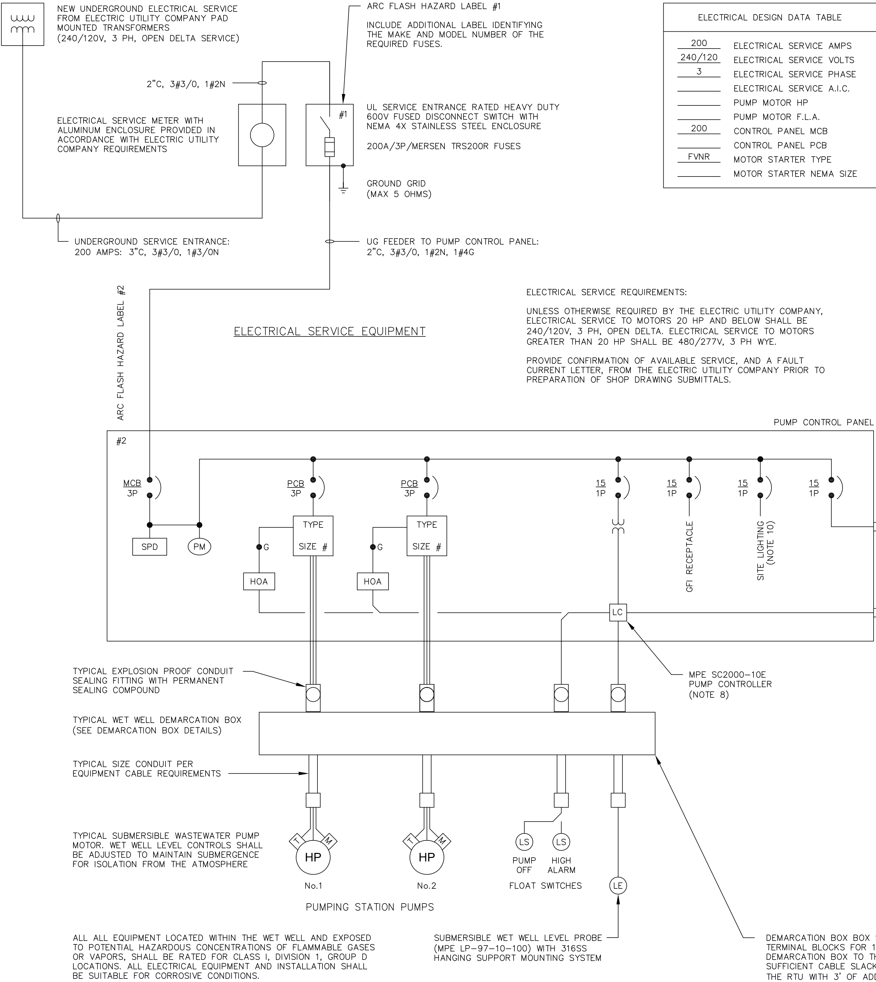
TYPICAL SJUCUD LIFT STATION – SINGLE LINE DIAGRAM
