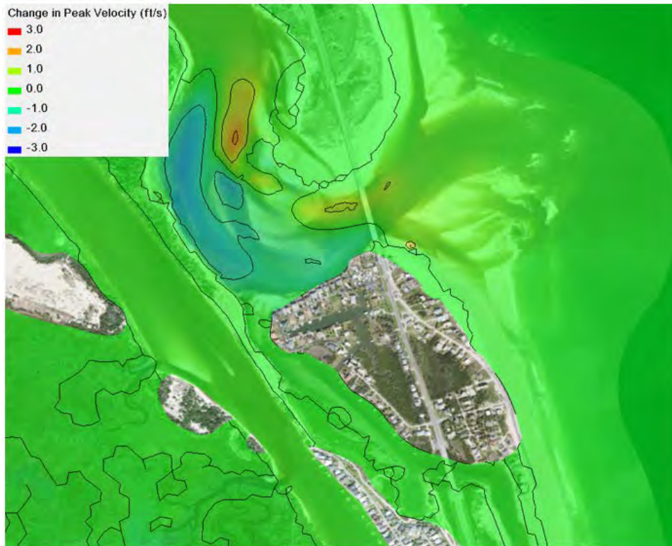
Figure 1.25 Change in Velocity within Inlet at Peak Flood Flow – Scenario 4 vs. Existing Conditions
