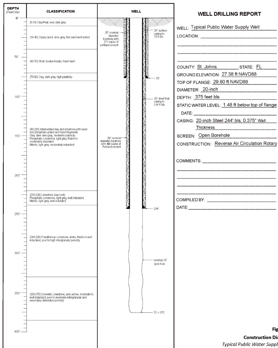
Figure 6: Typical Public Supply Well Detail
